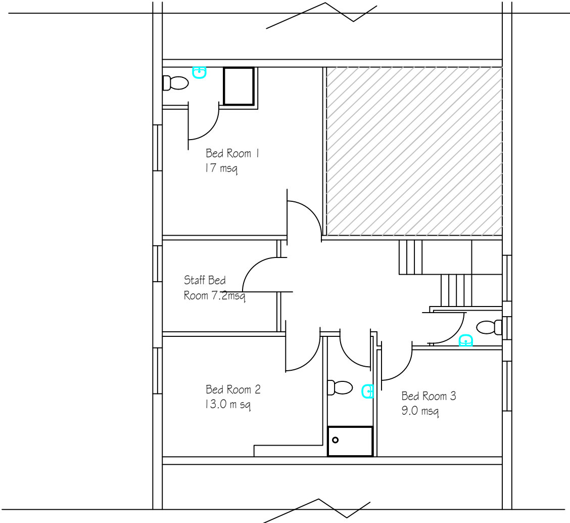
Proposed 1st Floor Plan
