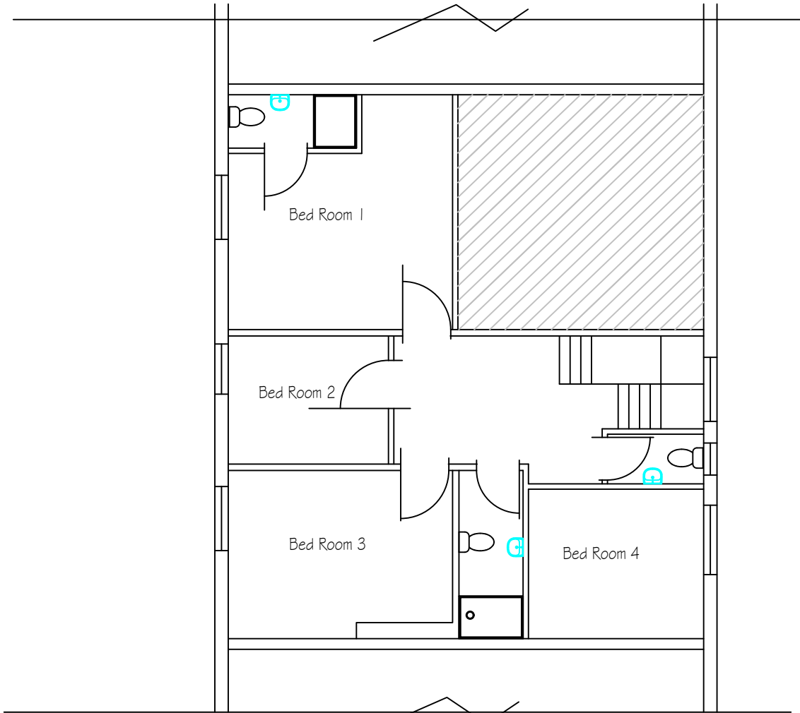
Existing 1st Floor Plan
