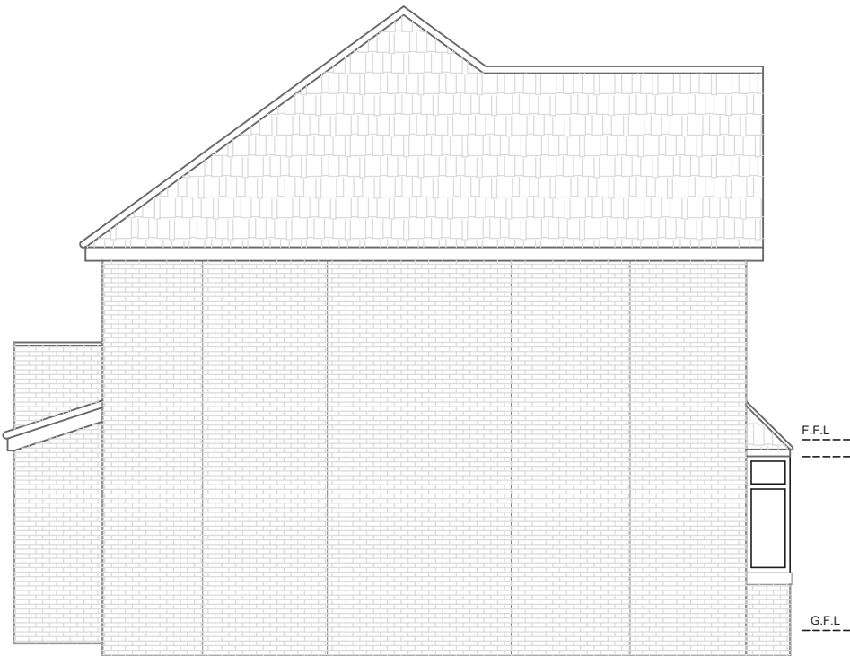
EXISTING SIDE ELEVATION (SOUTH )
