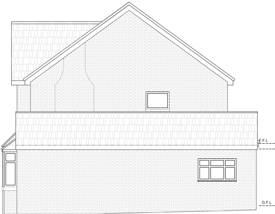
EXISTING SIDE ELEVATION (NORTH)
