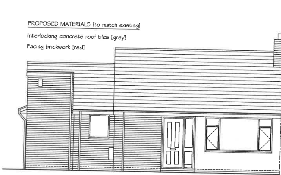
PROPOSED SOUTH WEST ELEVATION
