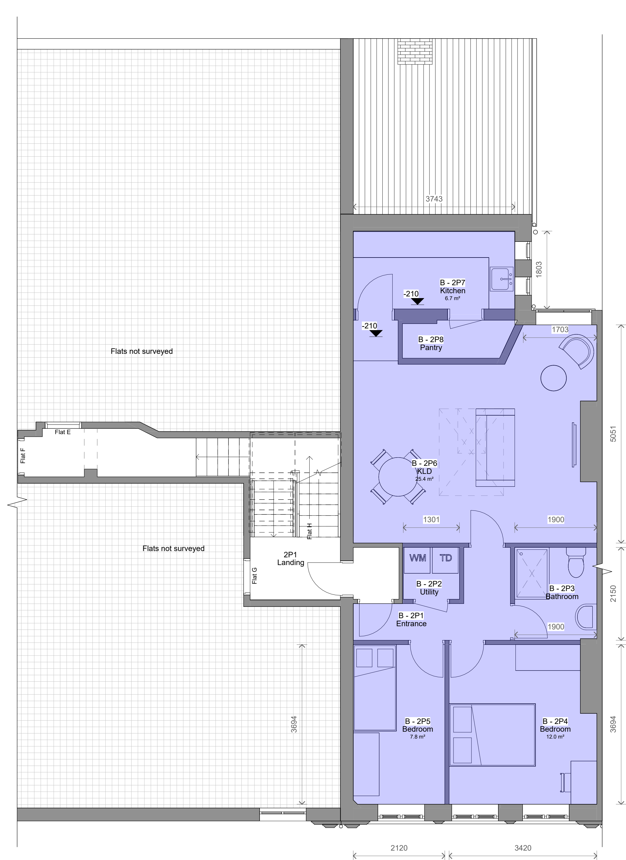
2 Level 2 - Proposed 1 : 50
