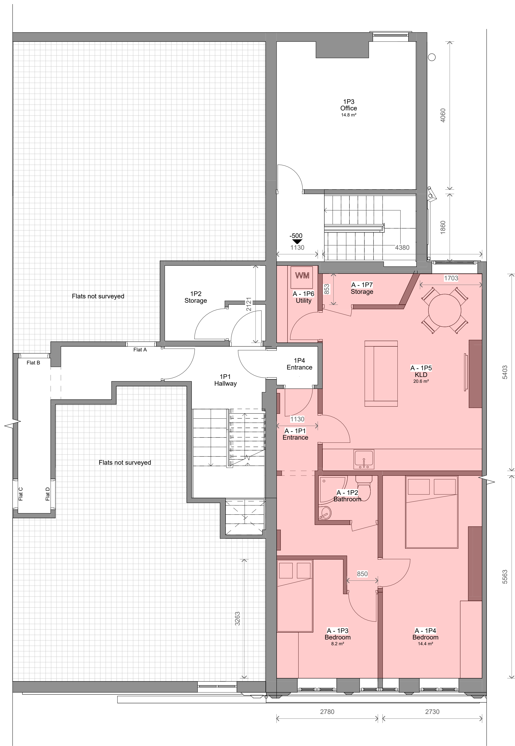
1 Level 1 - Proposed 1 : 50
