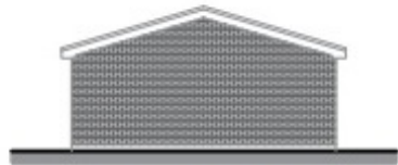
Proposed East Elevation Scale (1:100)
