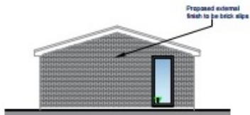
Proposed West Elevation Scale (1:100)
