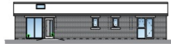
Proposed North Elevation Scale (1:100)
