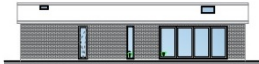
Proposed South Elevation Scale (1:100)
