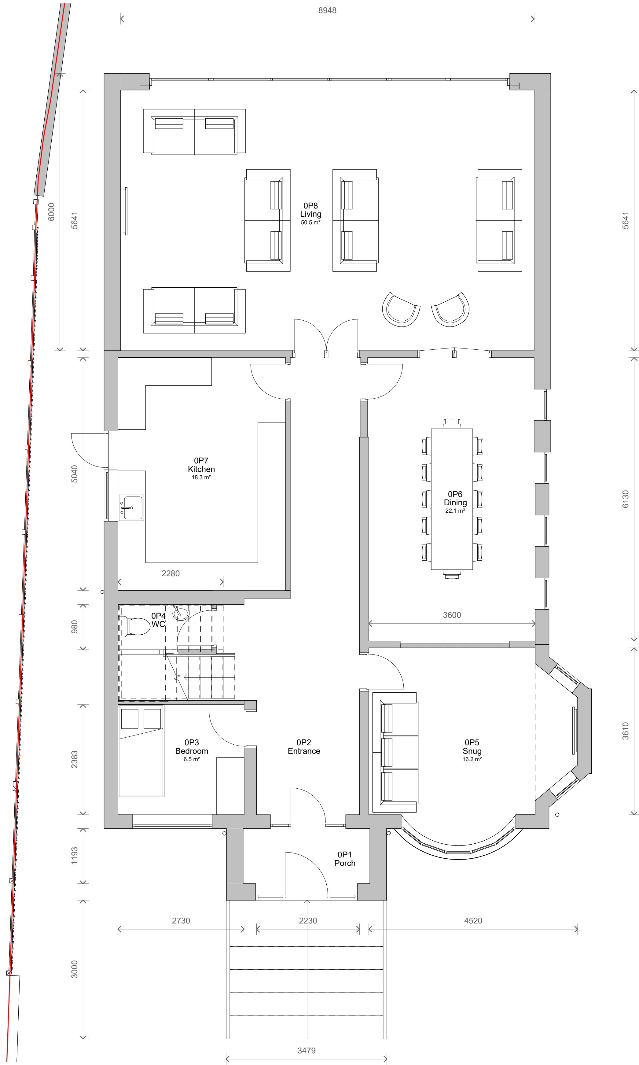
1 Level 0 - Proposed 1 : 50
