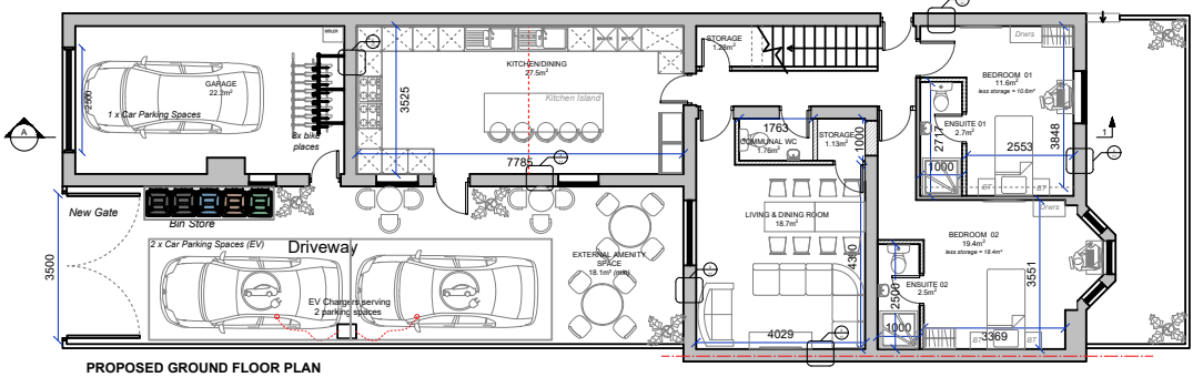
KEY PLAN: 1:200 @ A3
