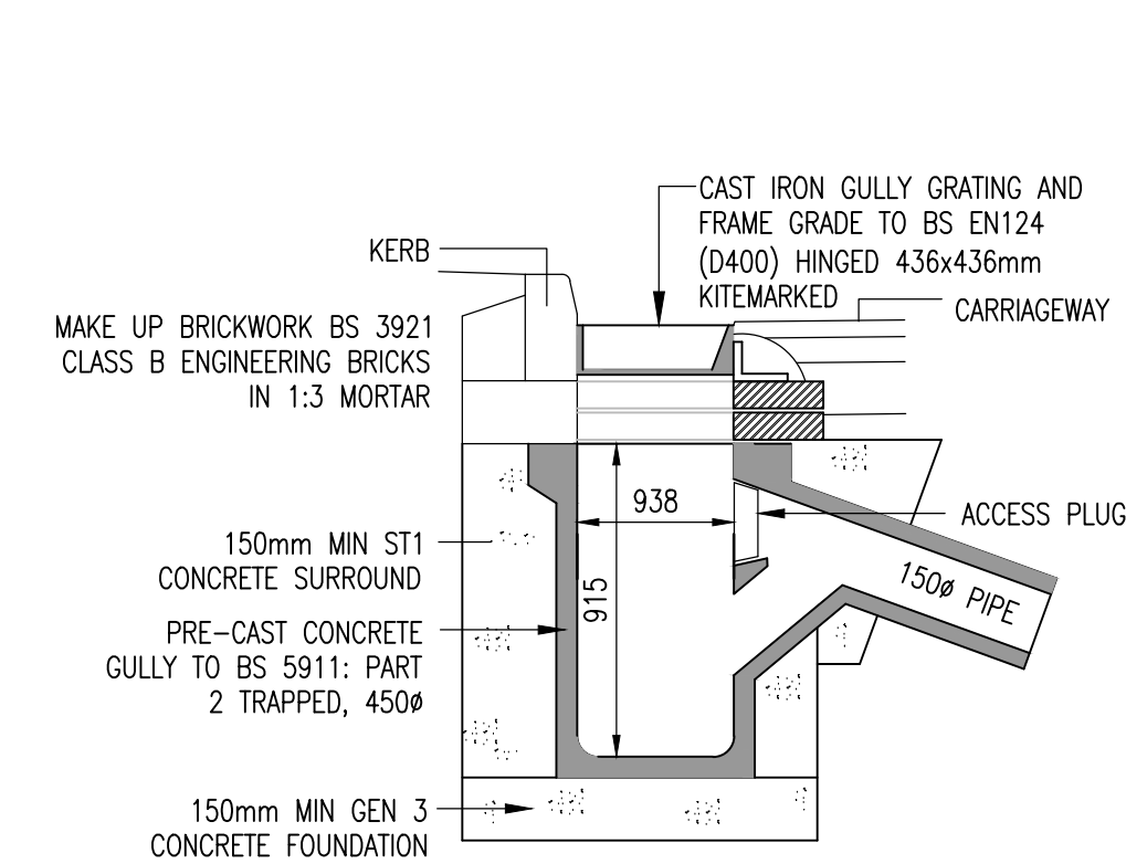
TYPICAL PRECAST CONCRETE ROAD GULLY DETAIL
