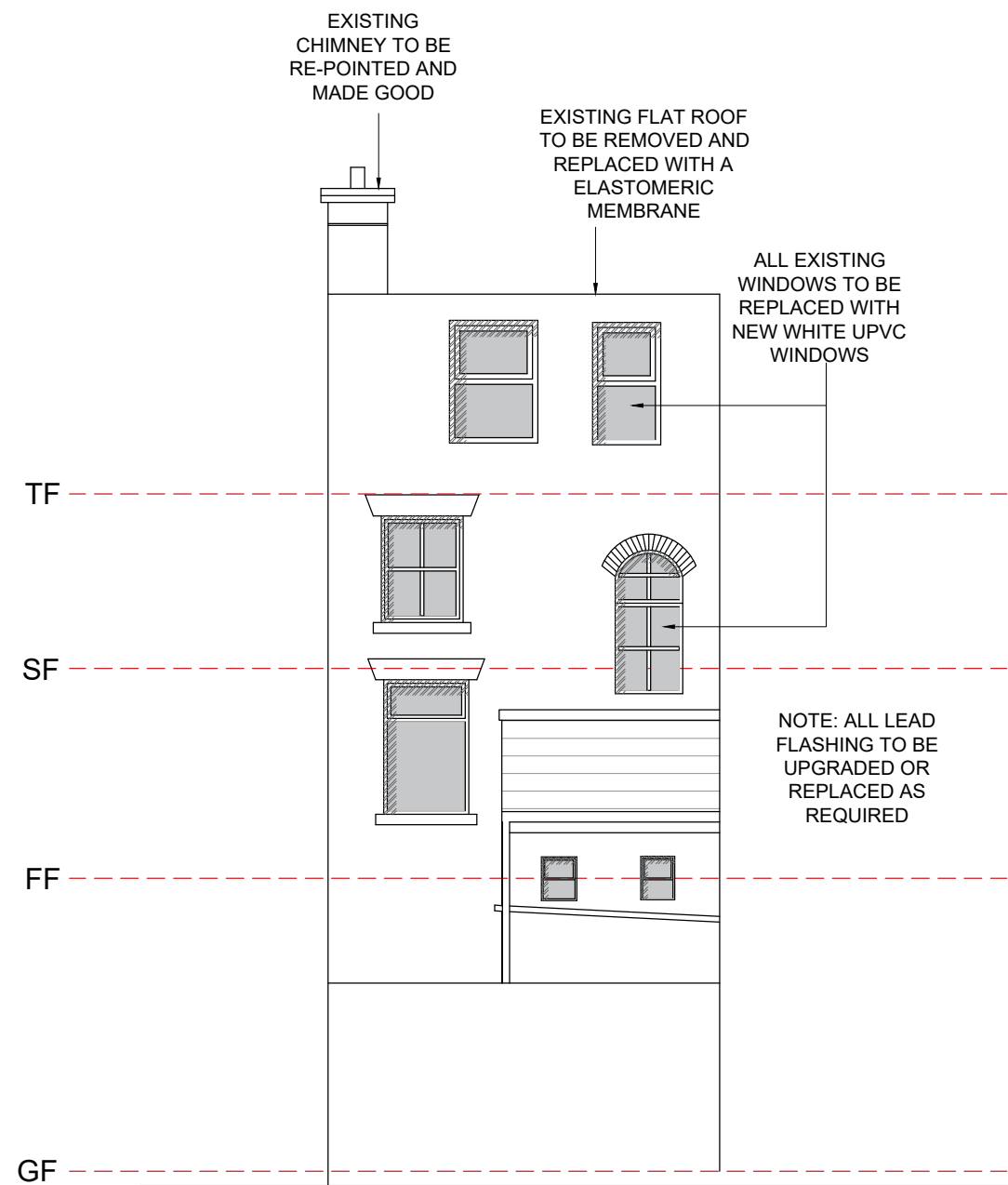
REAR ELEVATION
