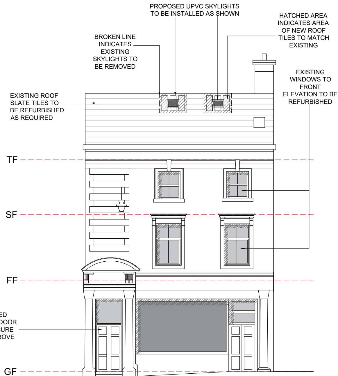
FRONT ELEVATION
