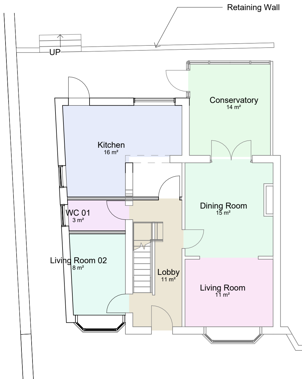
Ground Floor as Proposed 1 : 100
