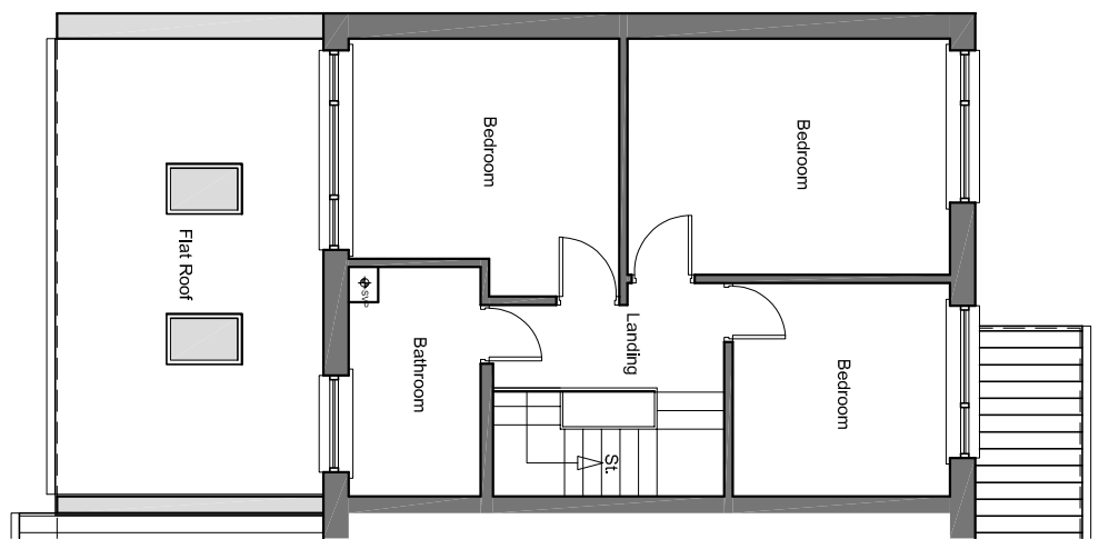
Proposed First Floor Plan 1:100
