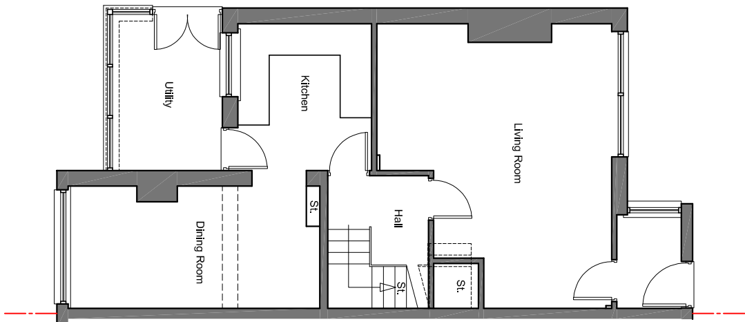
Proposed Ground Floor Plan 1:100
