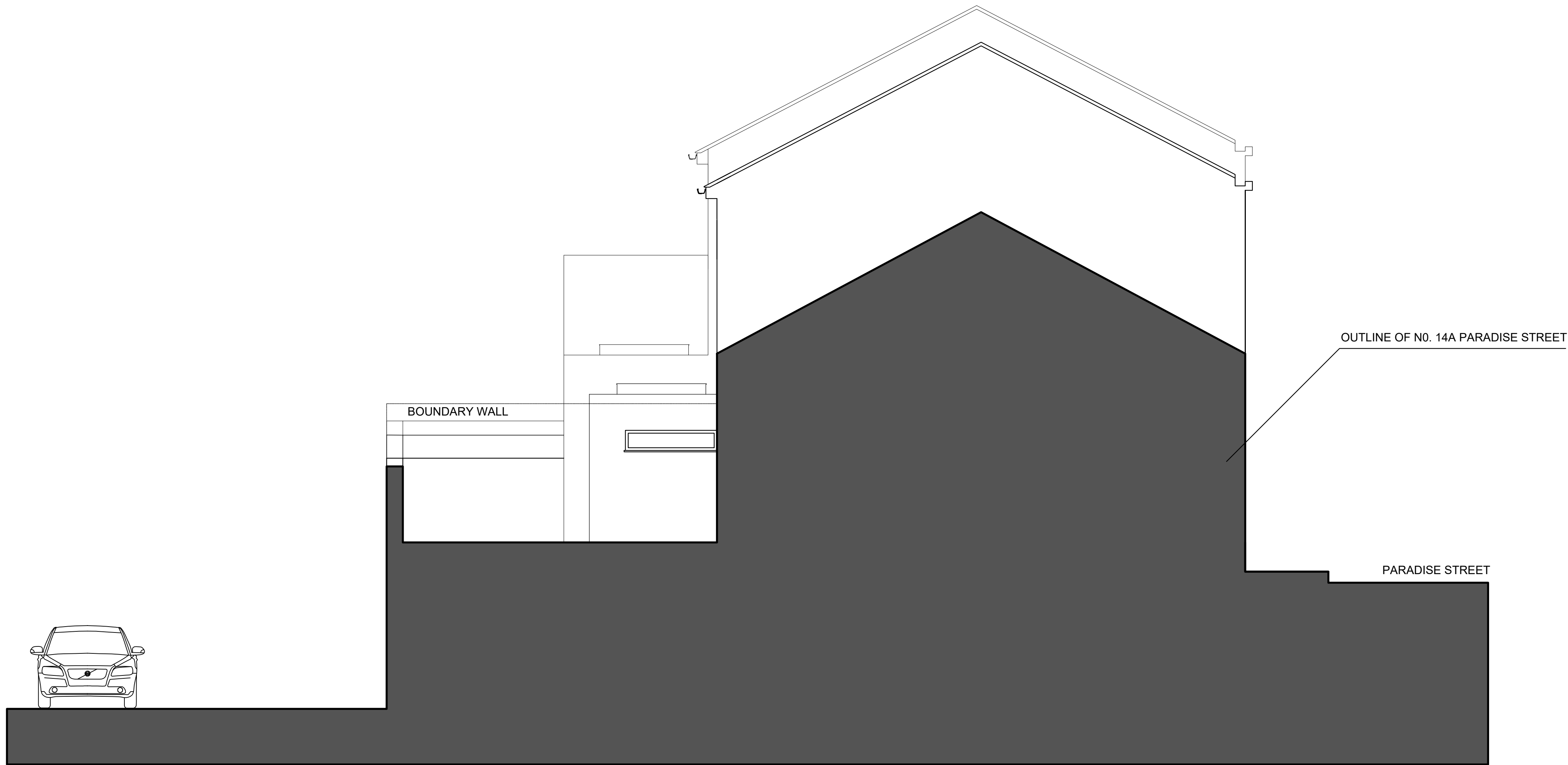
PROPOSED GABLE ELEVATION
