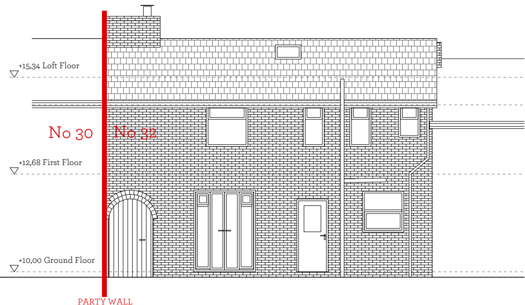
Elevation South
