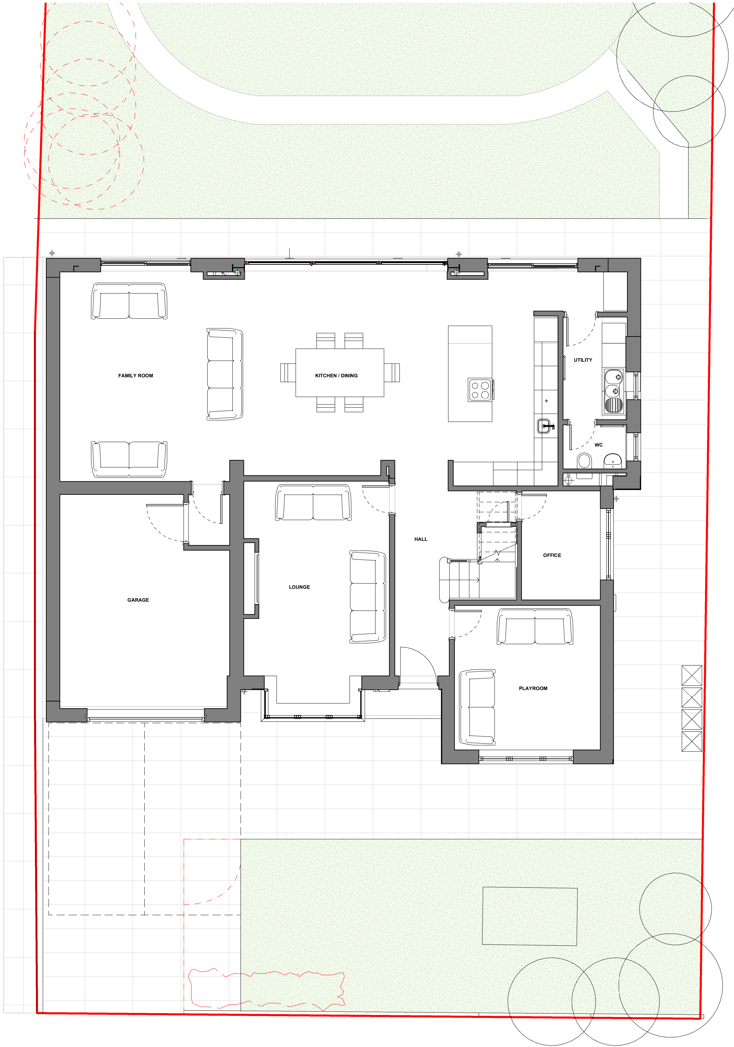
1 Level 0 - Proposed GA Plan 1 : 50
