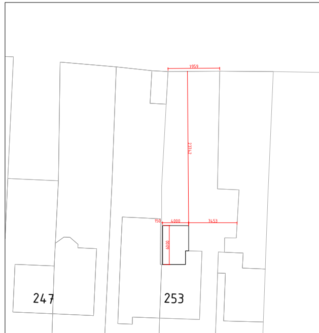
BLOCK SETTING OUT PLAN
