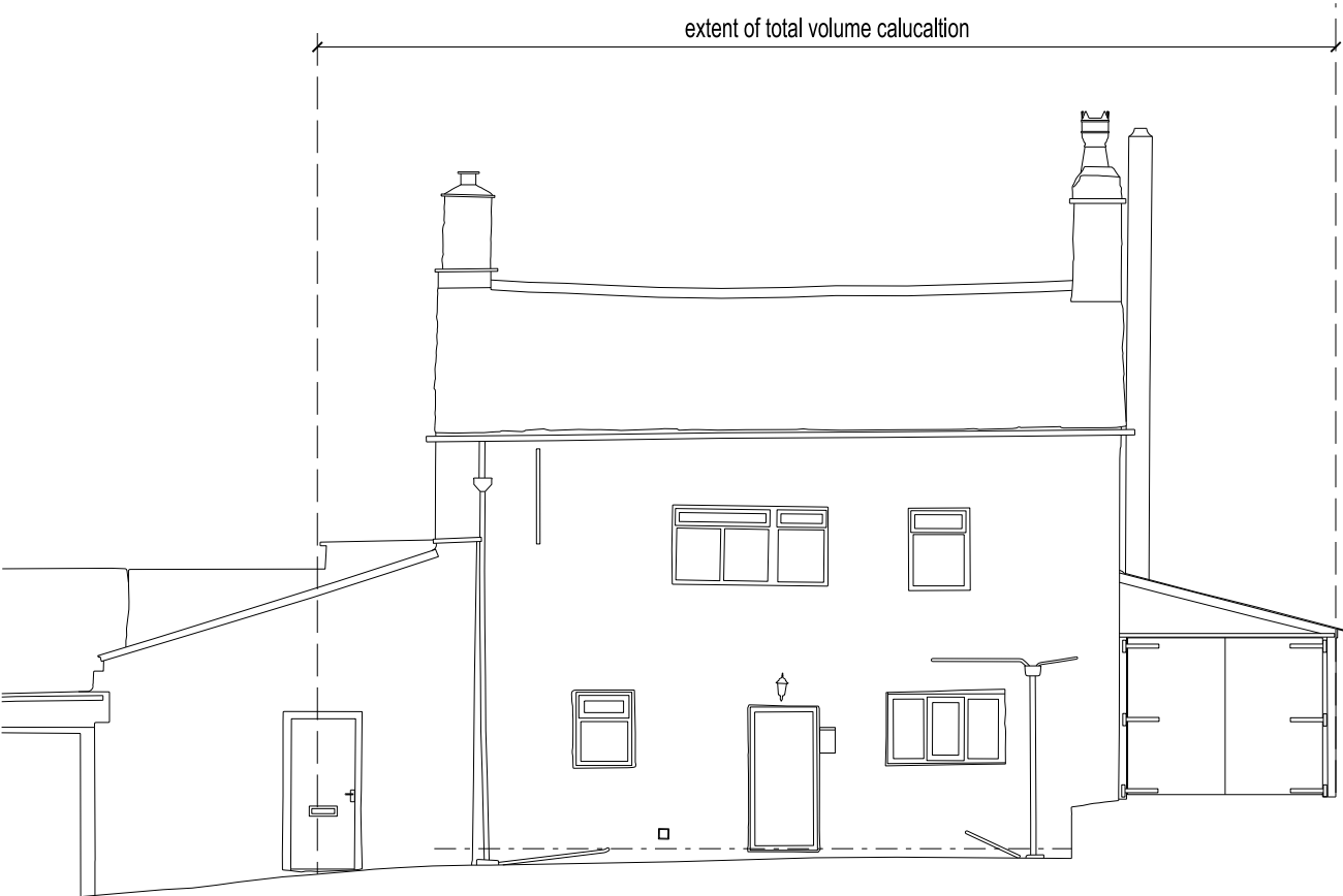
FRONT (NORTH) ELEVATION
