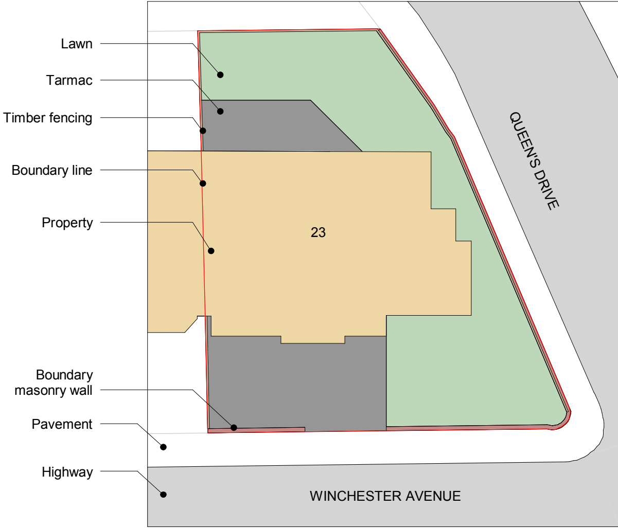
2. Site Layout - Proposed 1 : 200
