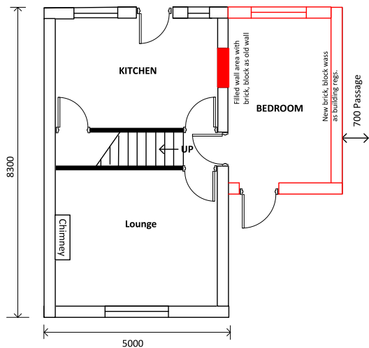
PROPOSED GROUND FLOOR
