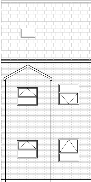
EXISTING REAR ELEVATION 1:100 @ A3
