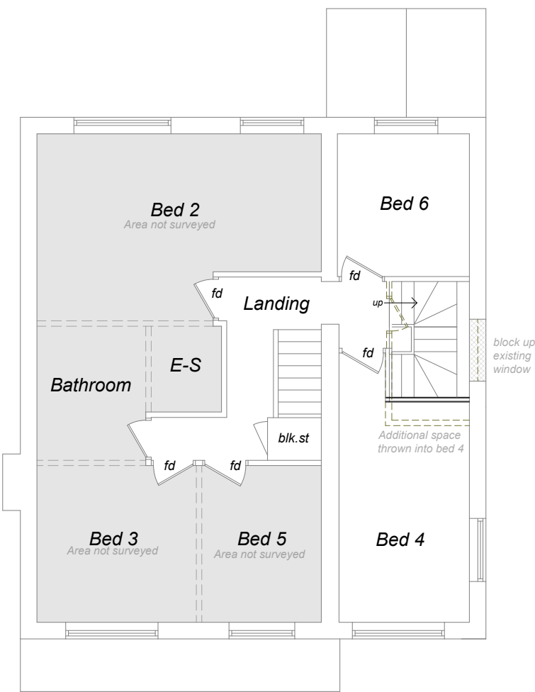
First Floor
