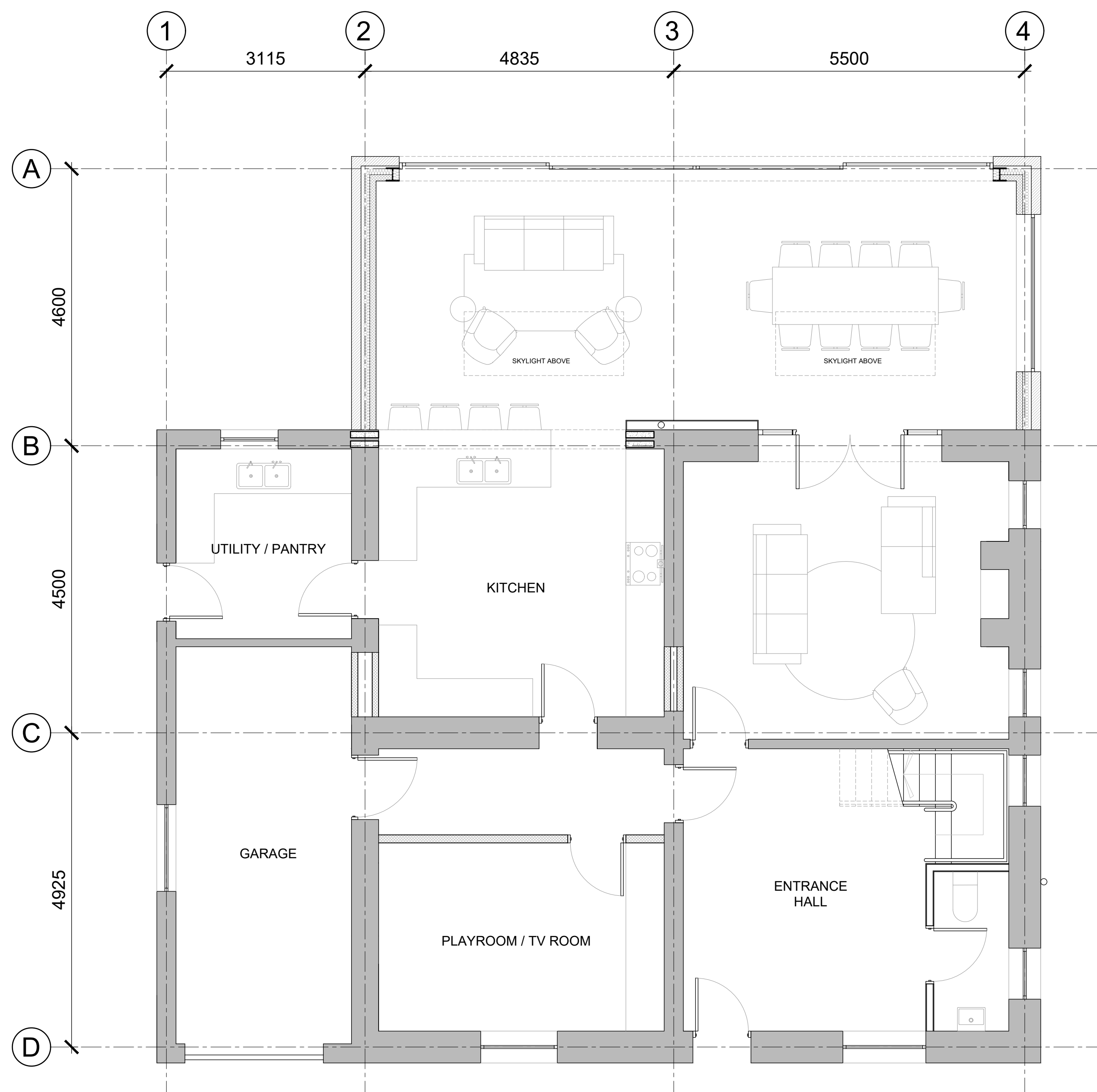
PROPOSED GROUND FLOOR
