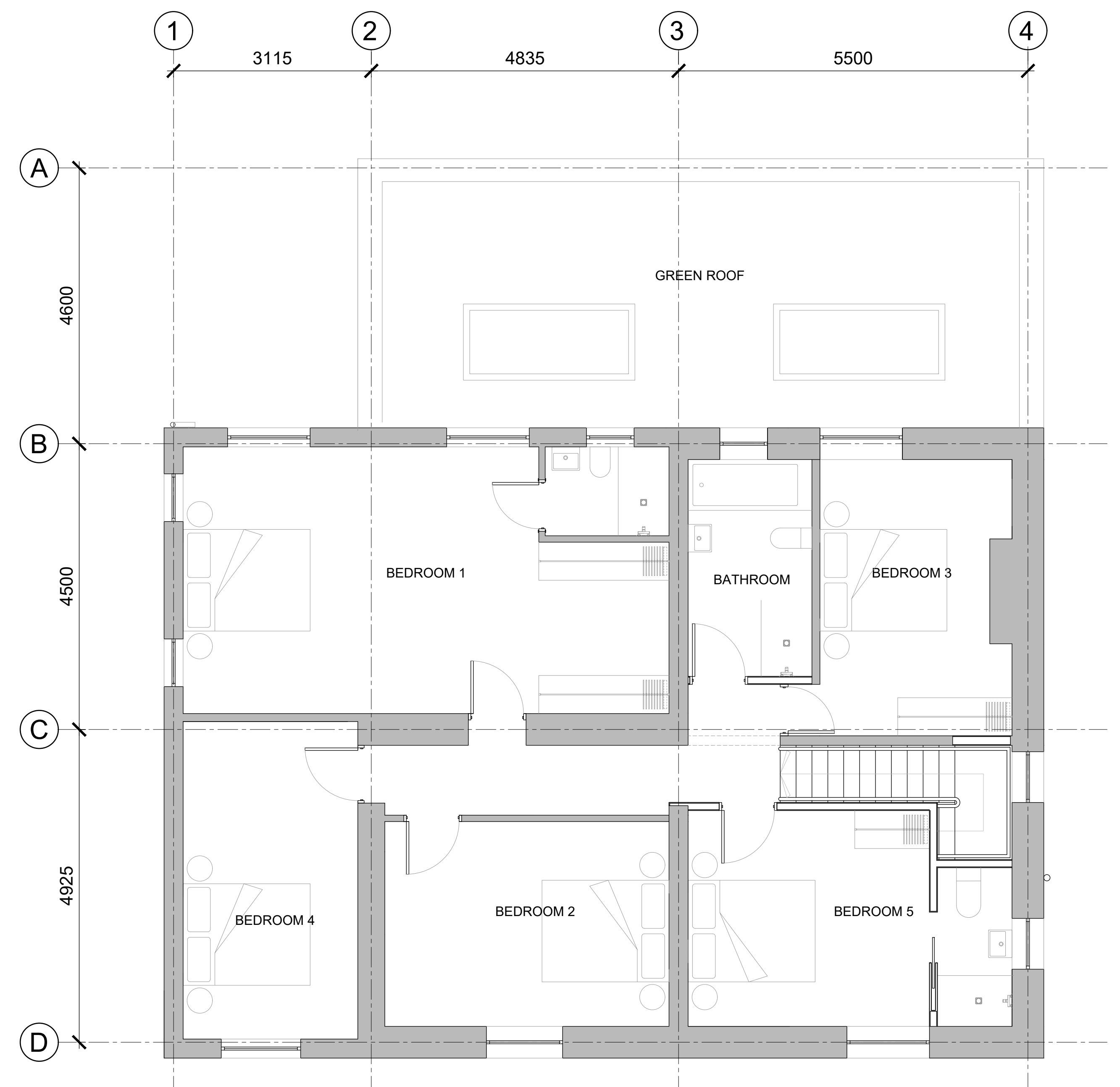
PROPOSED FIRST FLOOR
