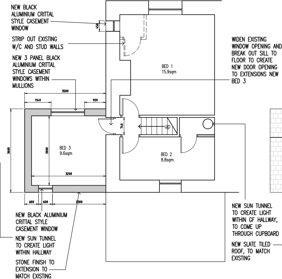
PROPOSED FIRST FLOOR PLAN 1:100 @ A3
