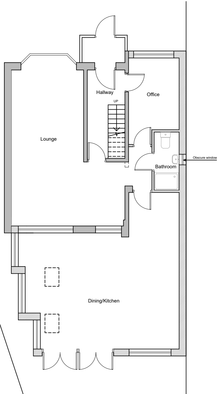
Approved Ground Floor Plan 1:100
