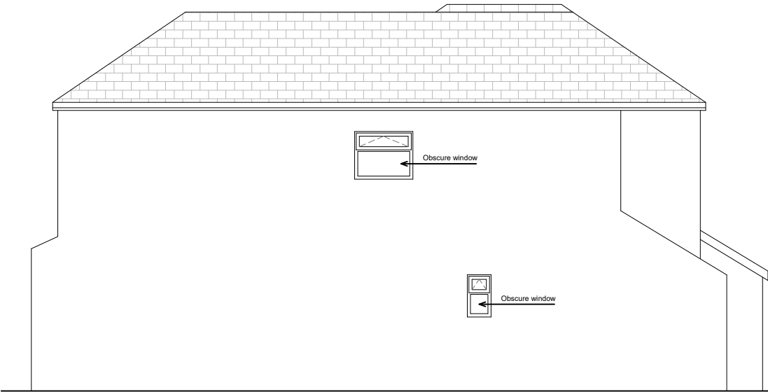
Approved Side Elevation 1 1:100
