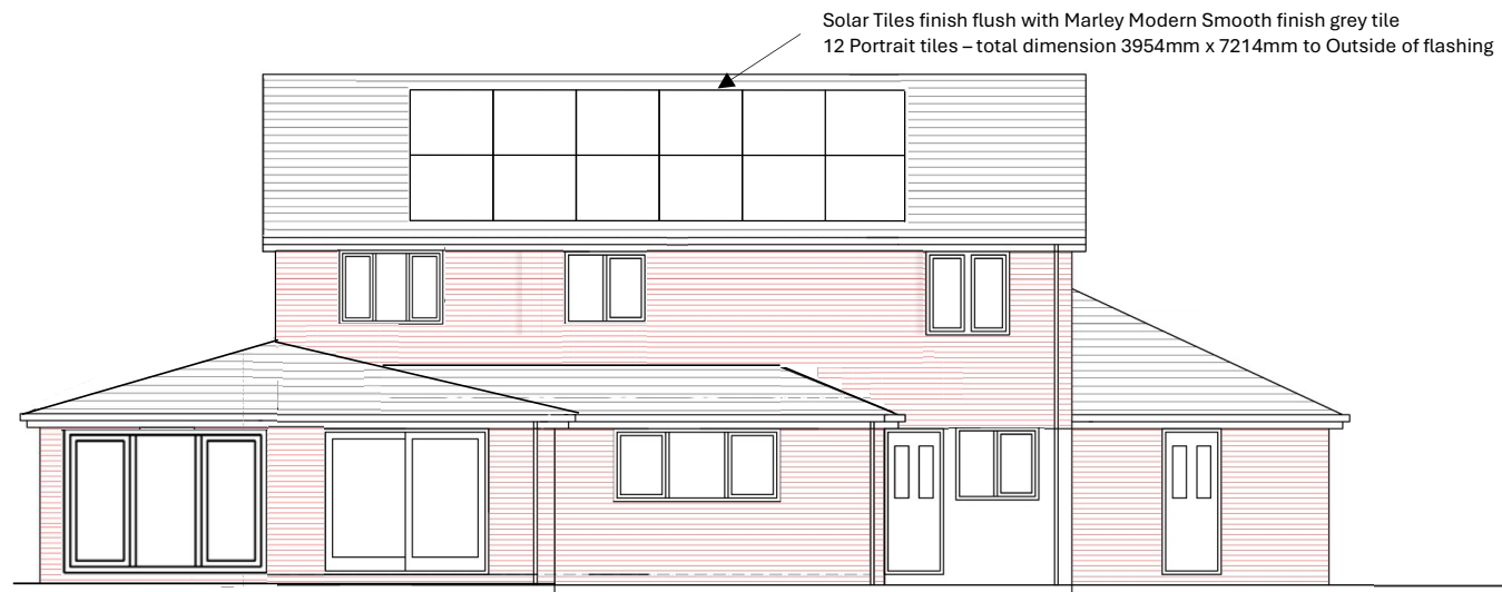
REAR ELEVATION
