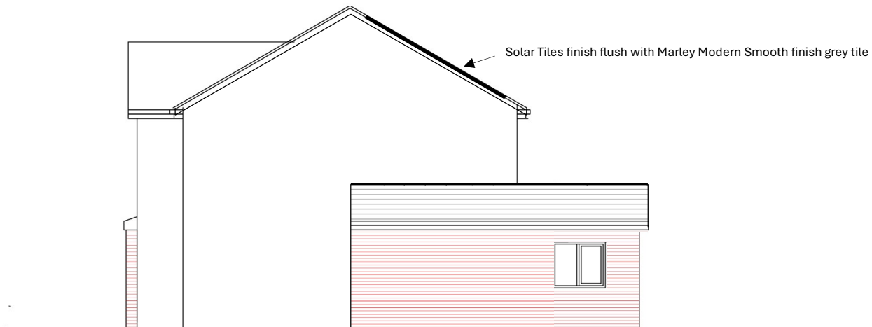
SIDE ELEVATION
