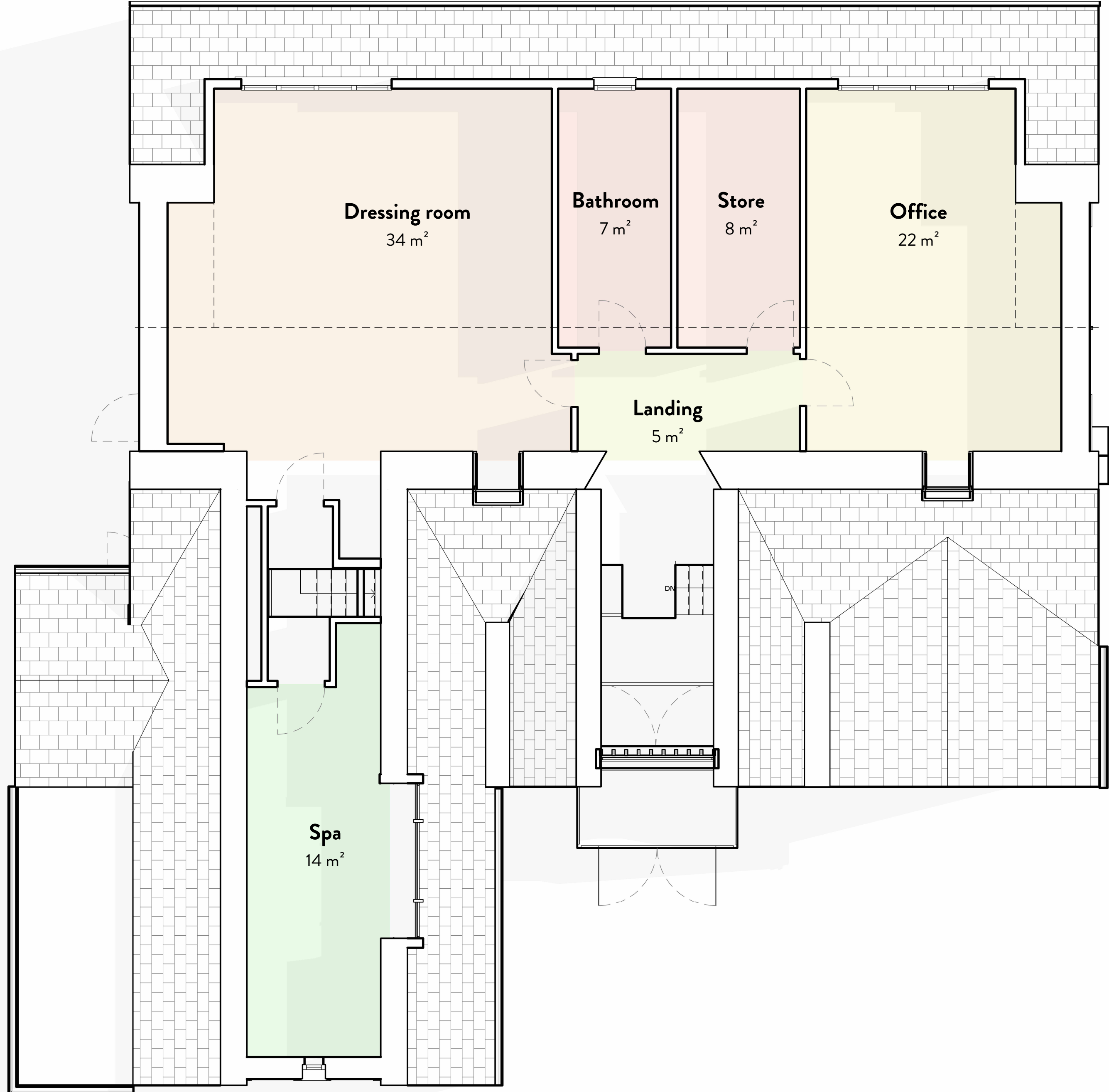
1 Loft - Proposed
