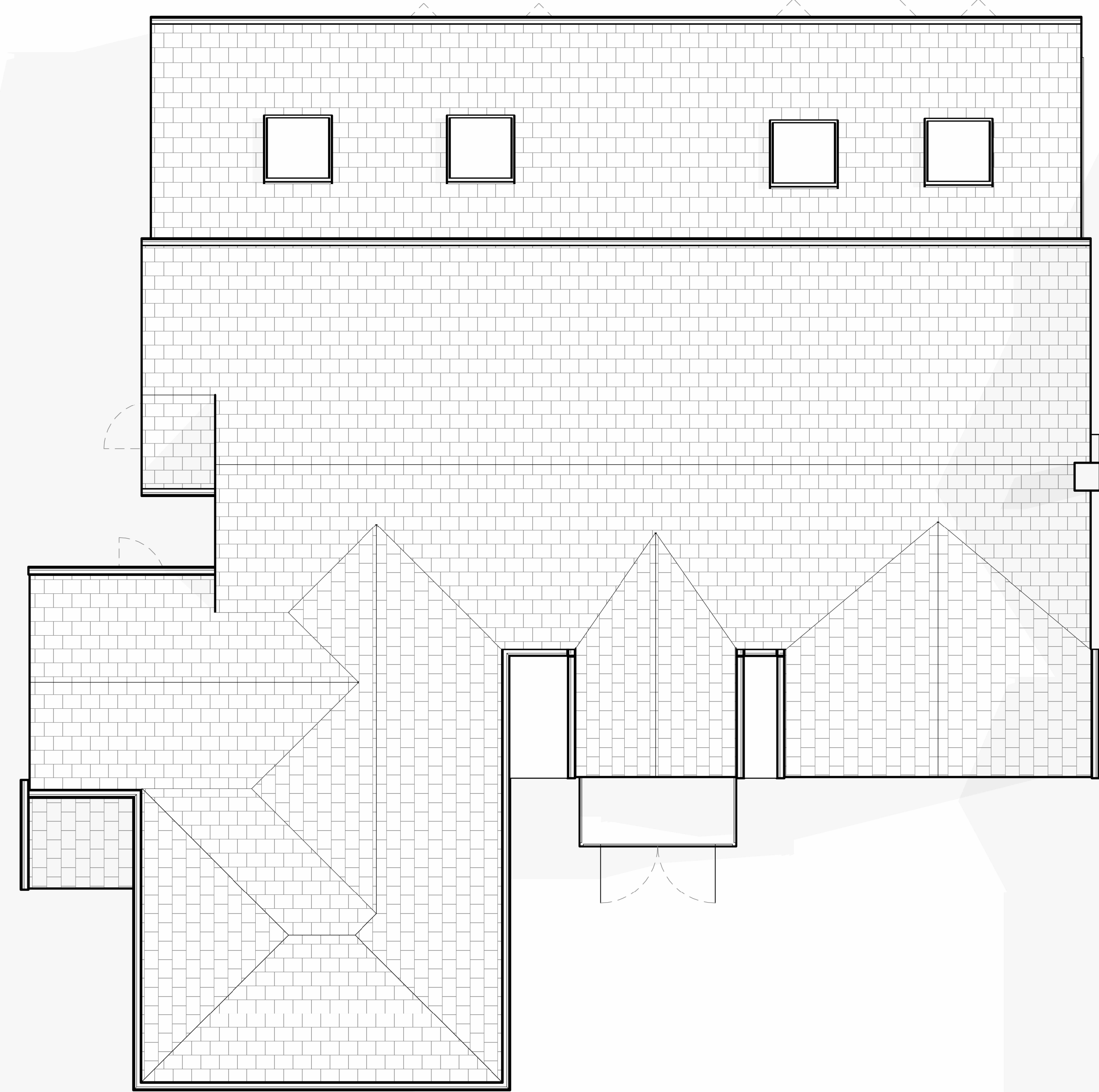
1 Roof - Existing
