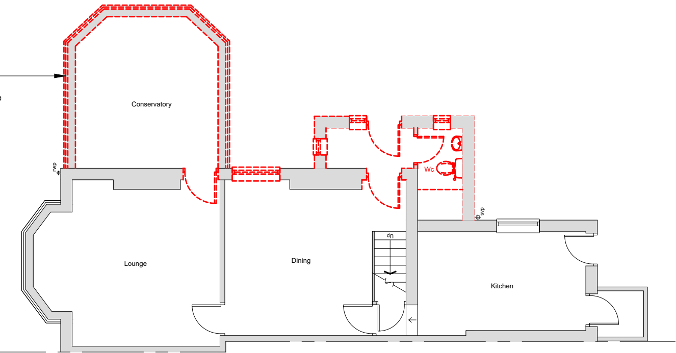
Existing GF Plan
