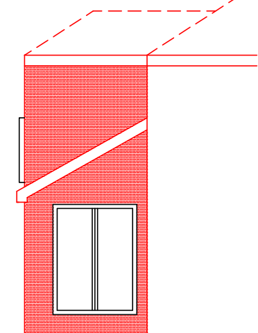
Proposed Inner Elevation
