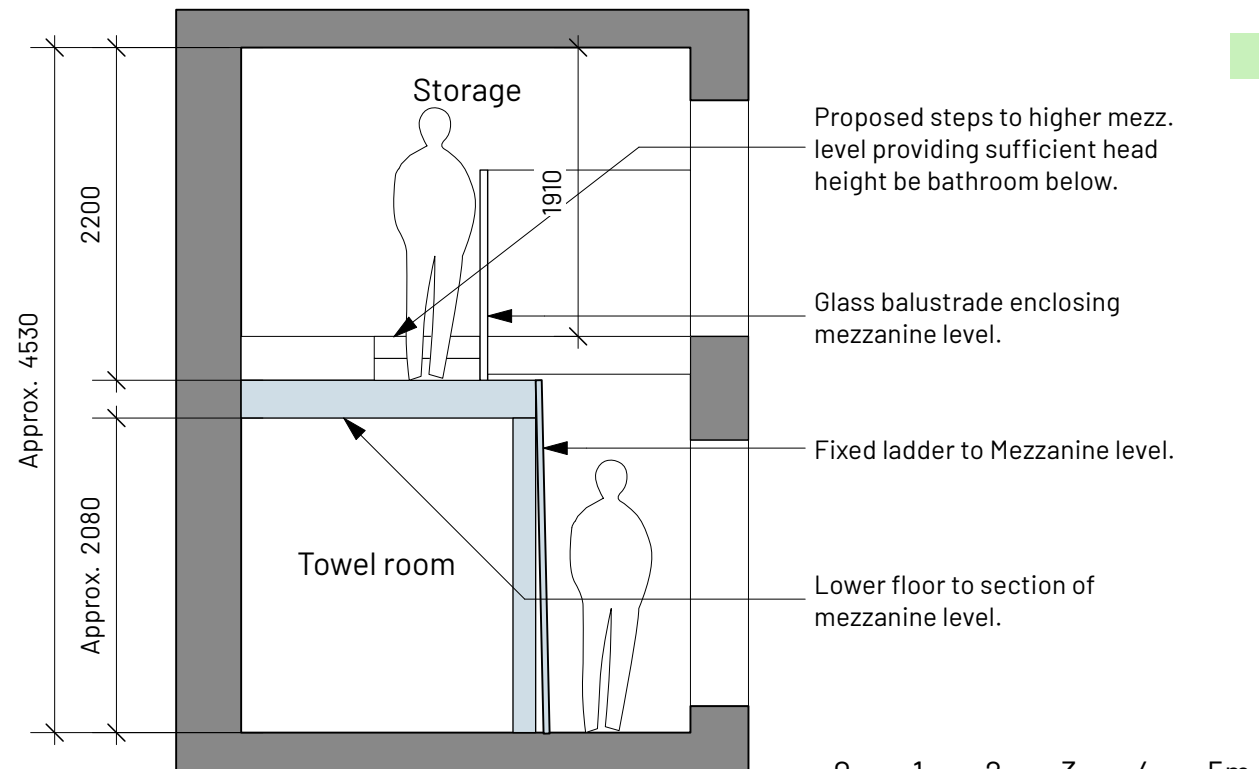
3 Section A-A Proposed Scale: 1:50
