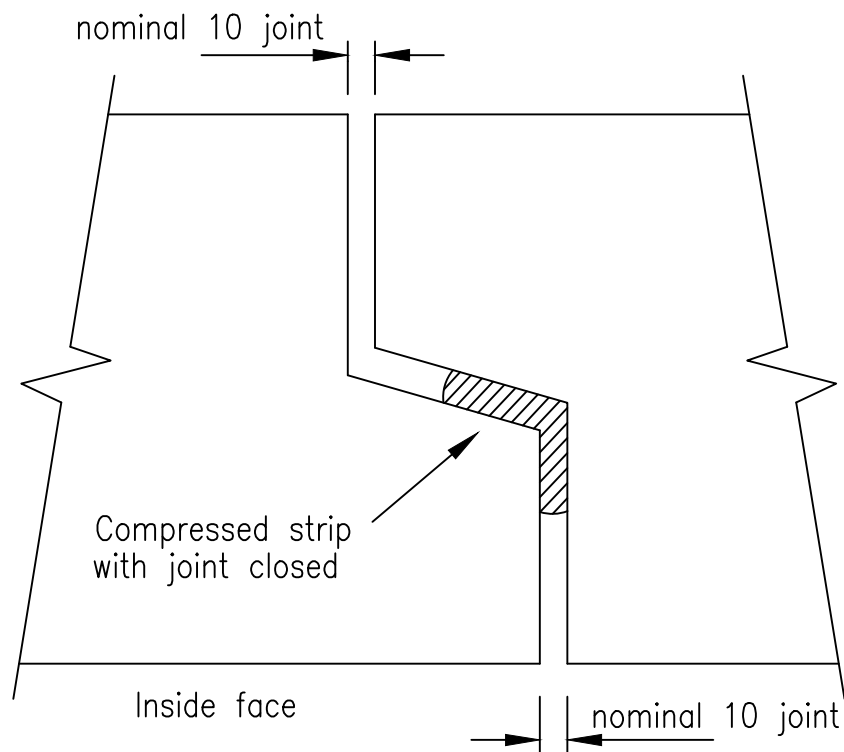
Closed joint
