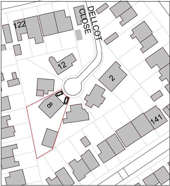
2 Site - Location Plan 1 : 1250
