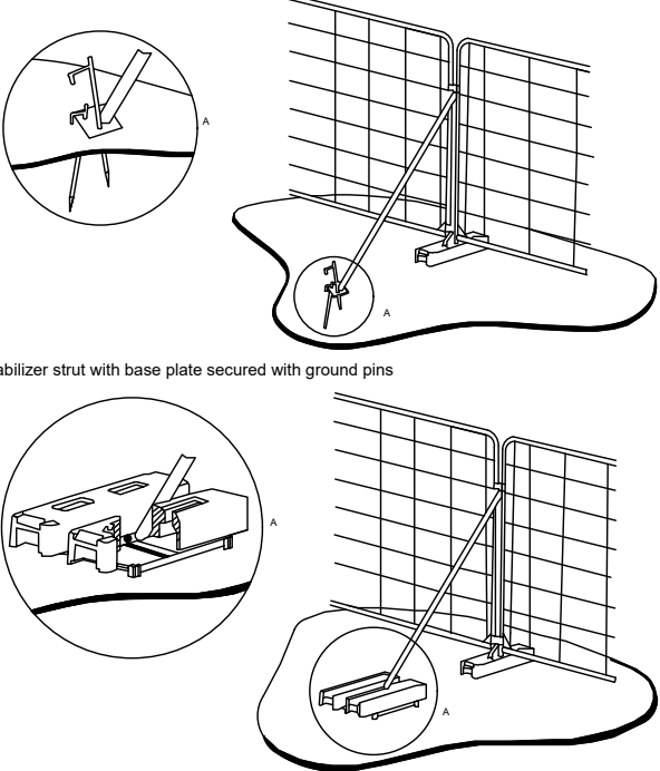
BS5837:2012 Figure 3 Examples of above-ground stabilizing systems
