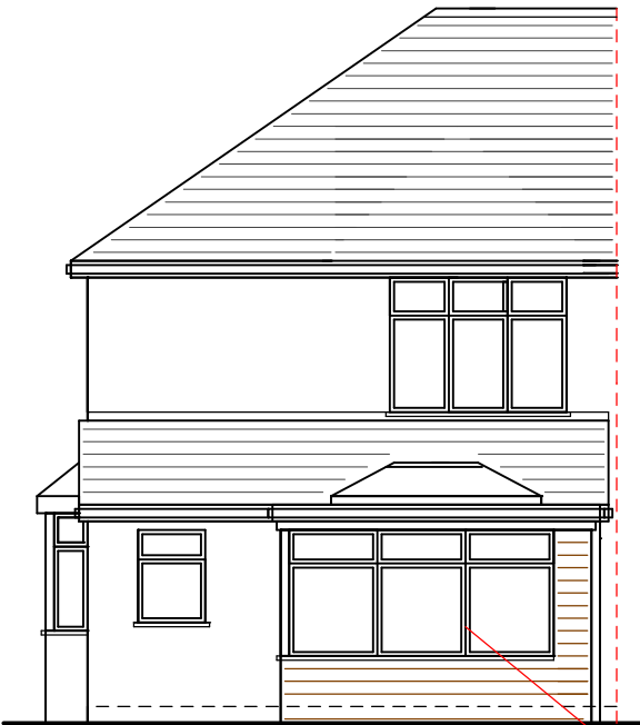
rear (southwest) elevation
