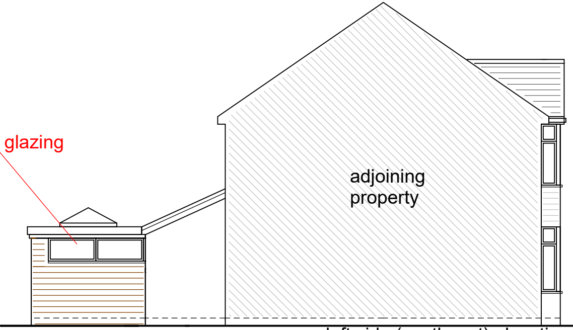
left side (southeast) elevation
