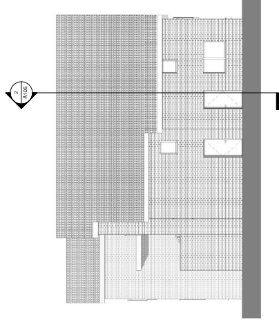
3 Proposed West Elevation 1 : 100
