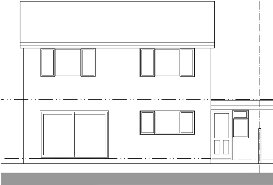
South East Facing Rear Elevation
