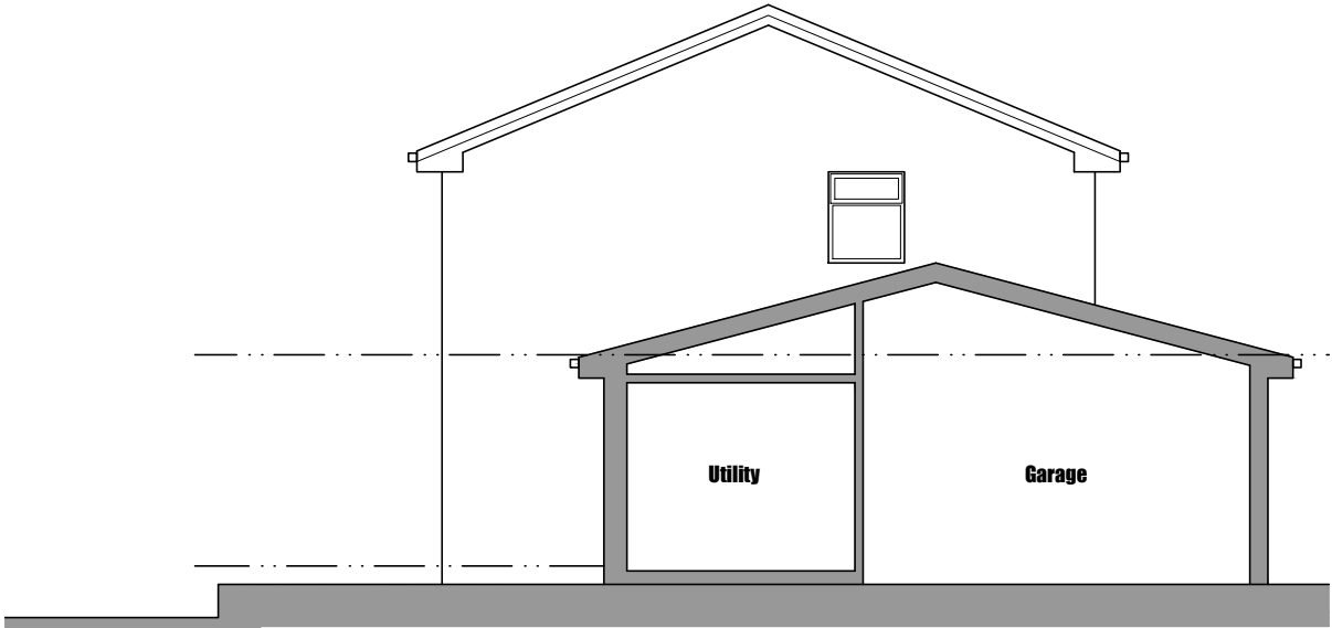
North East Facing Side Elevation
