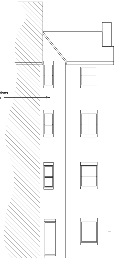
Existing North West Elevation (No change)
