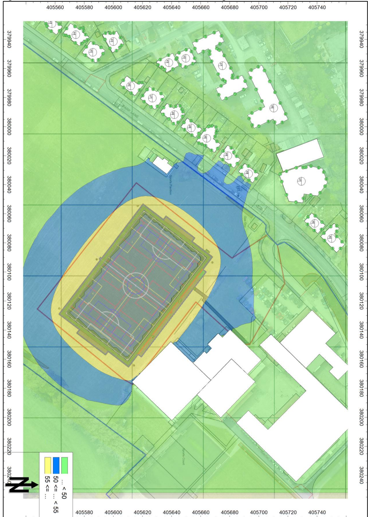
Figure 7: Predicted AGP Noise Emission 1.5 metres above the ground
