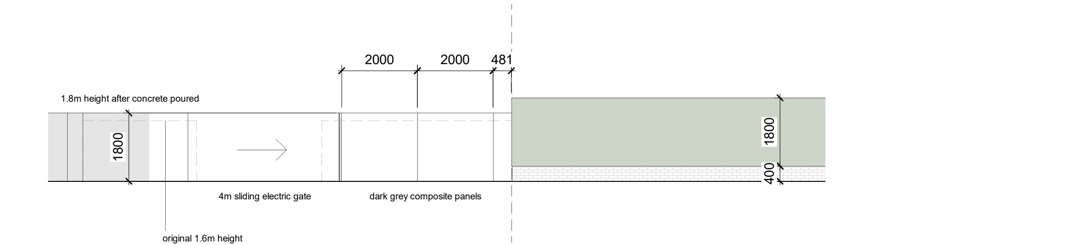
north elevation
