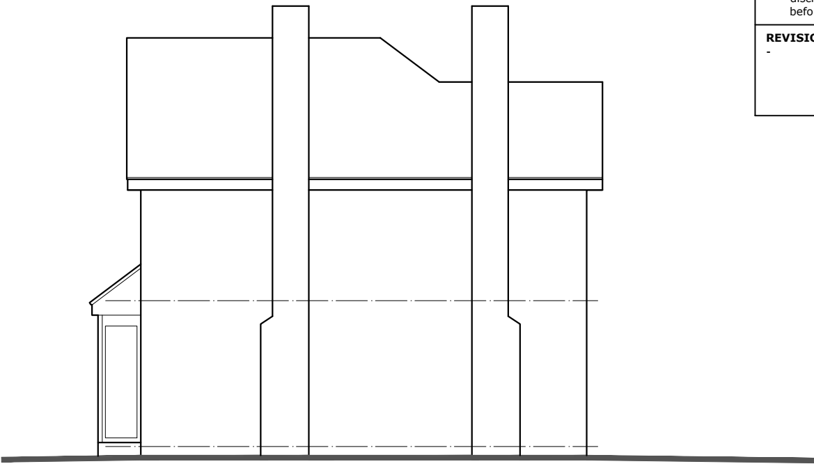
SIDE ELEVATION (facing Summerseat Lane)
