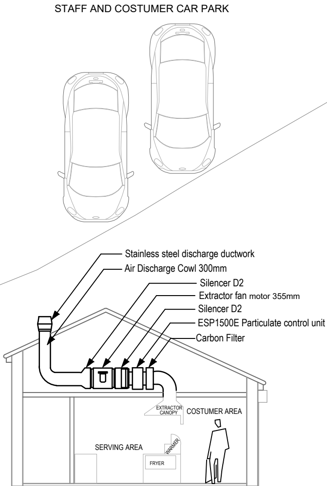
PROPOSED SECTION TO SHOW EXTRACTOR SYSTEM ARRANGMENTS
