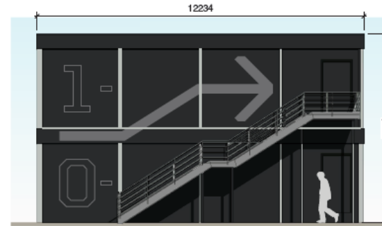
4 East Elevation 1 : 100
