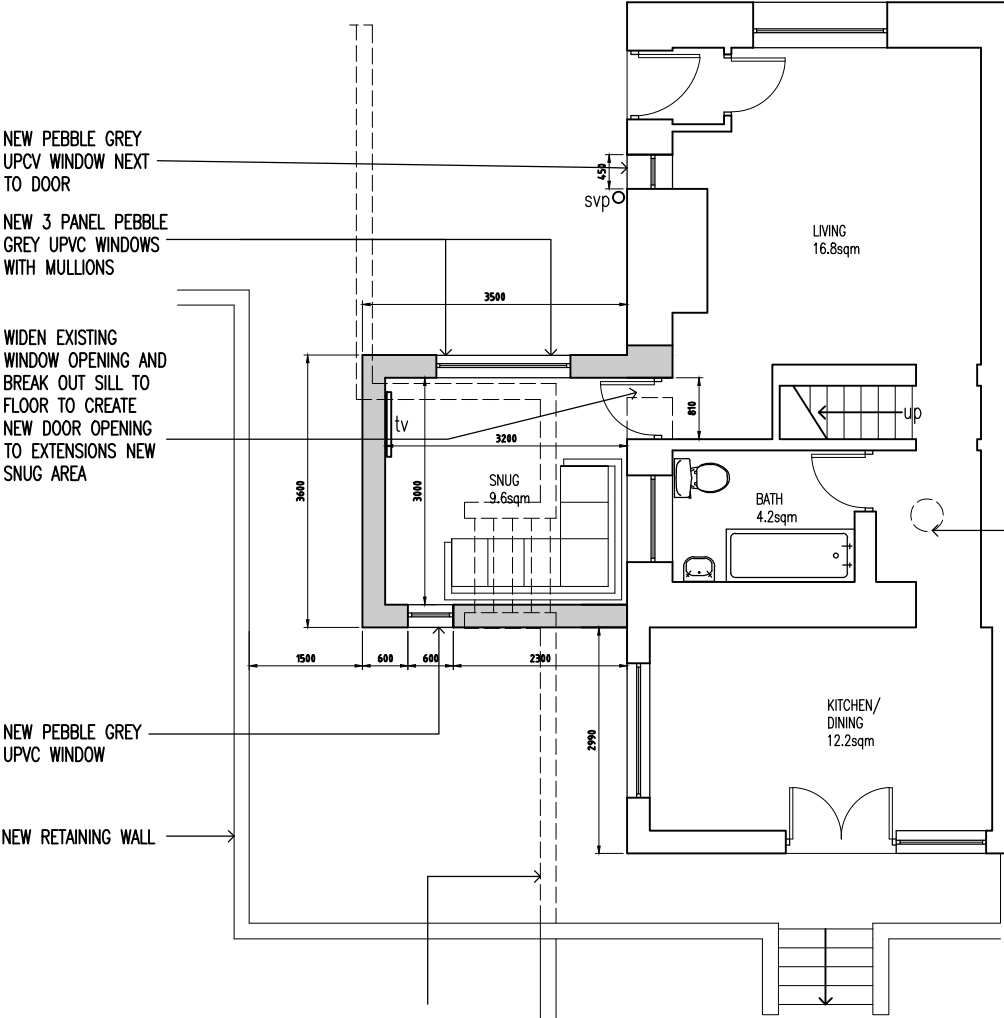
PROPOSED GROUND FLOOR PLAN 1:100 @ A3
