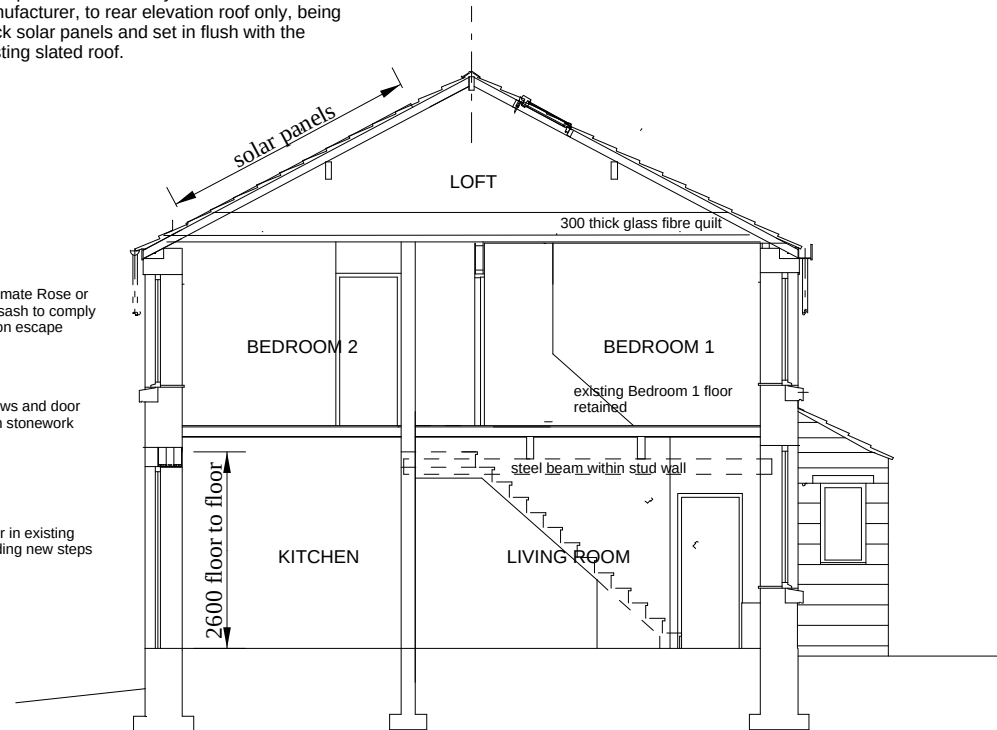
PROPOSED SECTION F-F
