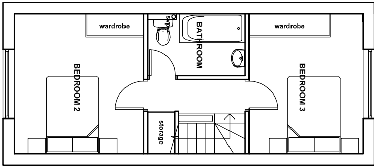
APPROVED DESIGN - SECOND FLOOR
