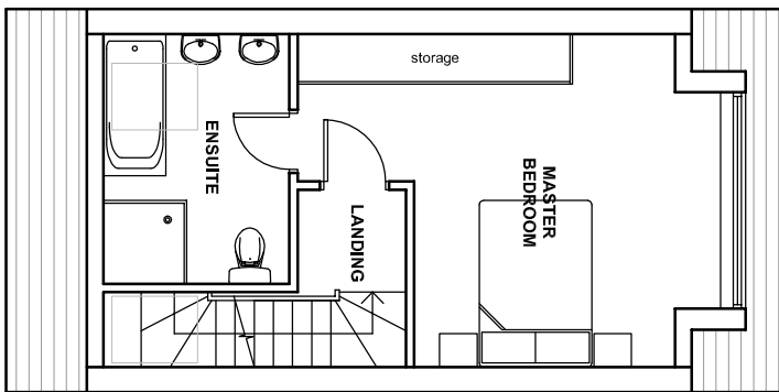
REVISED DESIGN - SECOND FLOOR
