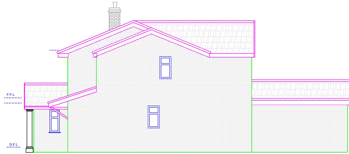
PROPOSED SIDE ELEVATION (NORTH)
