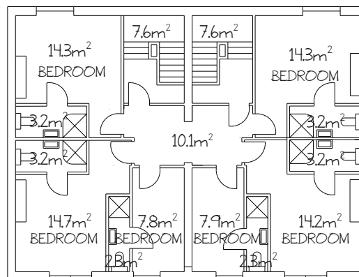
3 SECOND FLOOR 1:200 EXISTING
