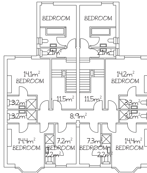
2 FIRST FLOOR 1:200 EXISTING
