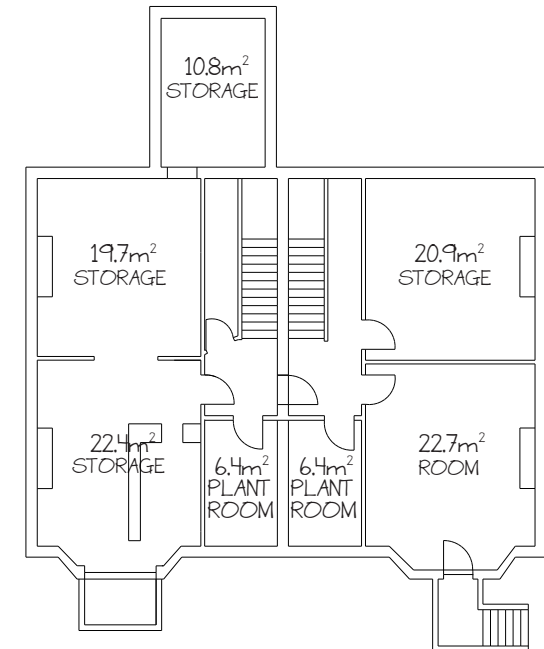
4 BASEMENT 1:200 EXISTING
