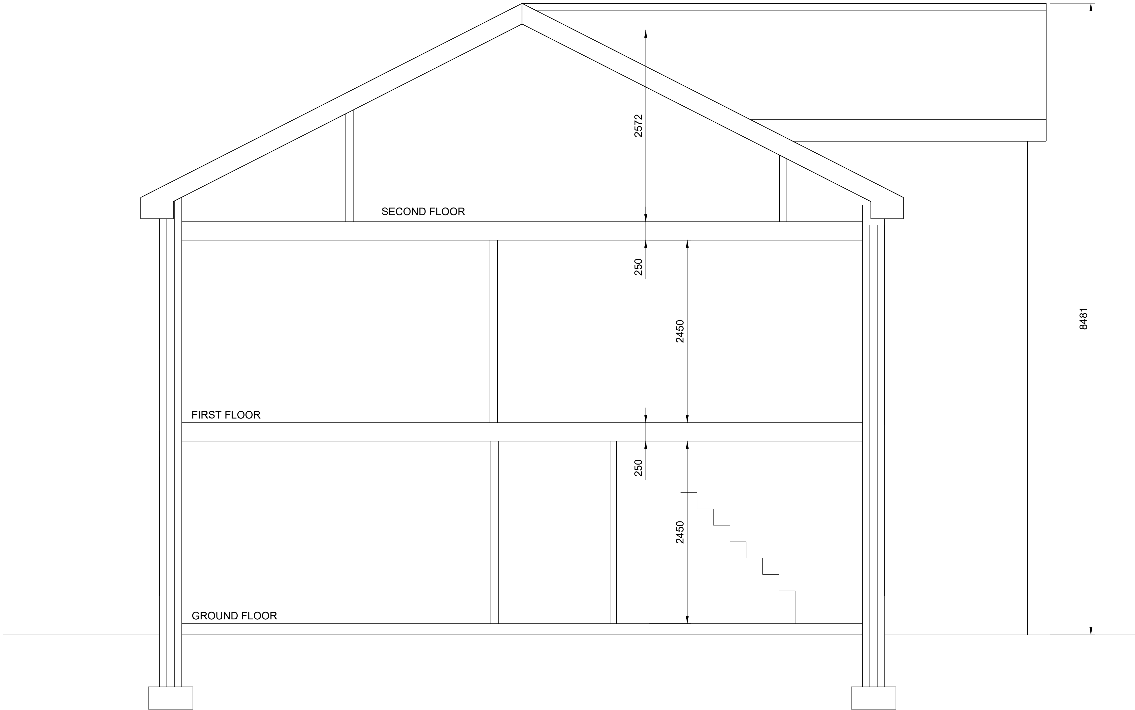
PROPOSED SECTION
