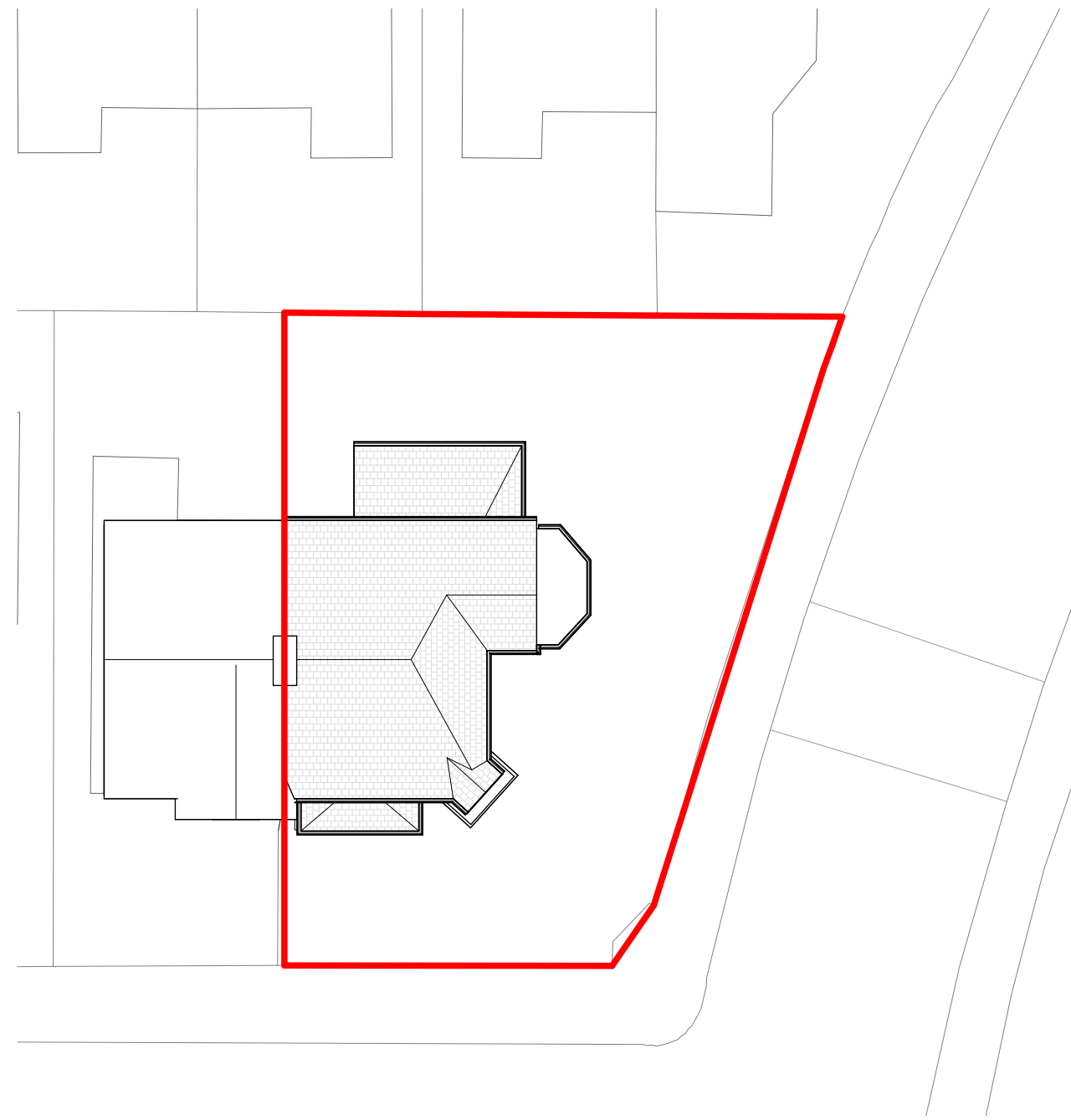
1 Block Plan - Existing 1 : 200
