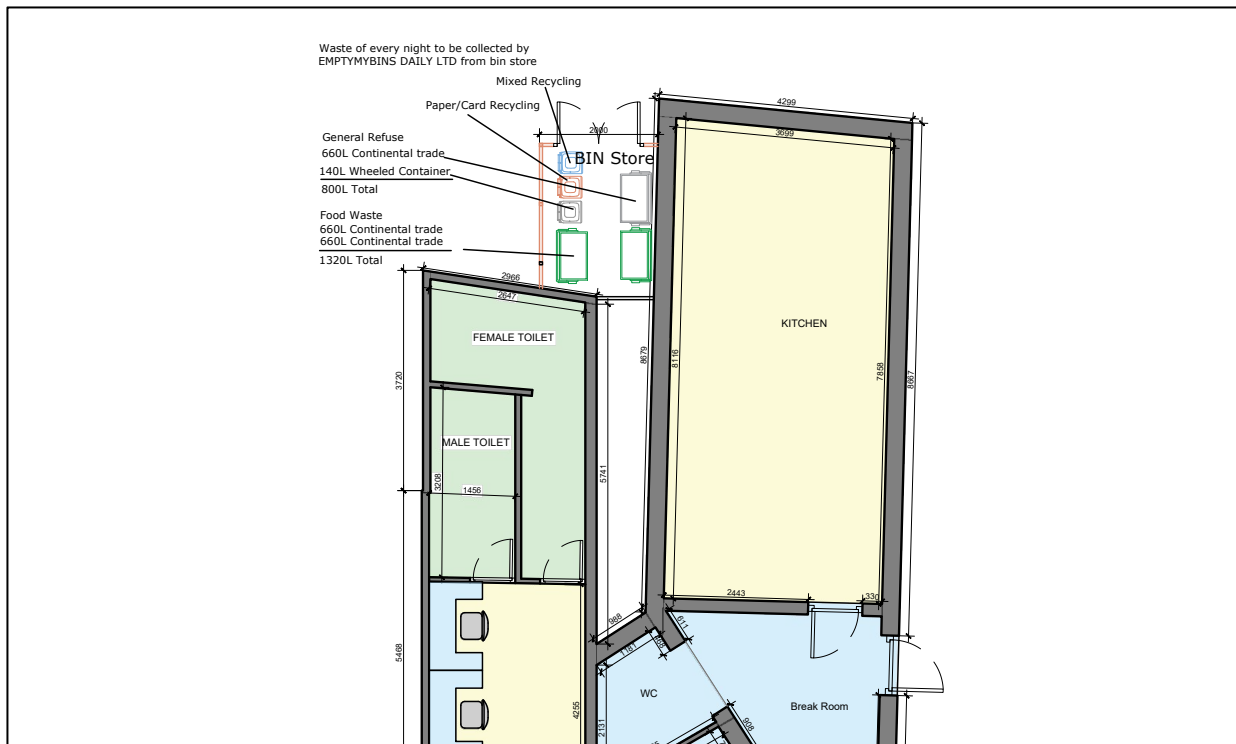
Proposed timber frame bin store: 12 Bolton St.
